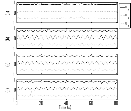
Fig. 9. Main directions \mathbf{u} = [u_x, u_y, u_z]^T of EHV variations found by ML for T_e delineation over: (a) clean simulated signal, (b) simulated signal including respiratory effect, (c) with noise for SNR = 30 dB and (d) with noise for SNR = 10 dB.
