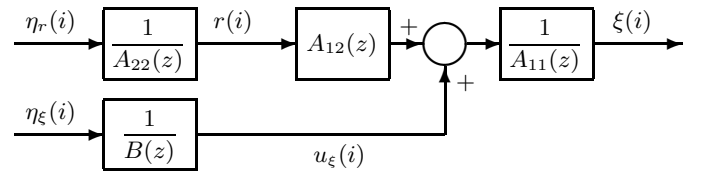
Fig. 5. Model of \xi(i) and r(i) interactions.
