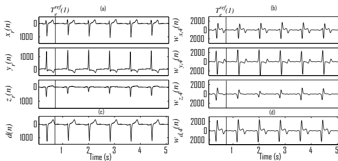
Fig. 3. Example of derived d(n) and w_{d,4}(n) signal. (a) Leads x_r(n) , y_r(n) and z_r(n) of VCG signal ( \mu V ) correspond to simulated signal affected by respiration (see section II-B1). (b) WT of leads x_r(n) , y_r(n) and z_r(n) in scale 4 (A.U.). (c) Derived ECG lead ( d(n) ) ( \mu V ). (d) Derived WT ( w_{d,4}(n) ) signal (A.U.). Vertical line corresponds to T_e .
