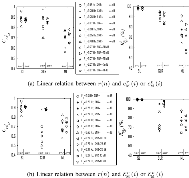
Fig. 8. Average coherence values and relative fractions of the total delineation error or additional error including the respiration. SNR = \infty stands for no simulated noise included.
