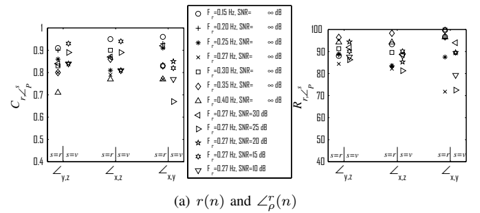
Fig. 10. Linear relation between r(n) and \angle_{\rho}^s(n) : average coherence values and relative fractions of explained variability.
